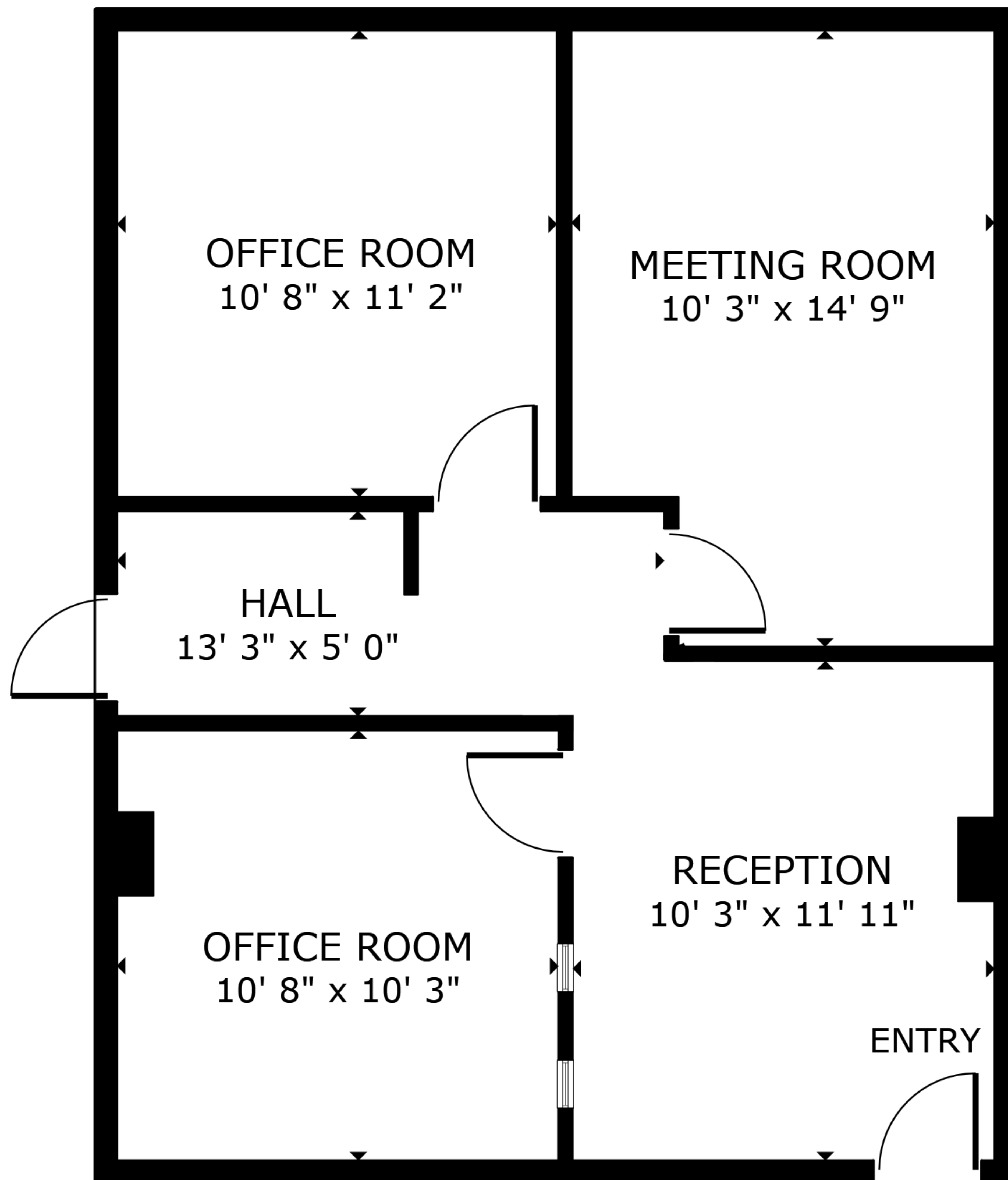
FLOOR PLAN
