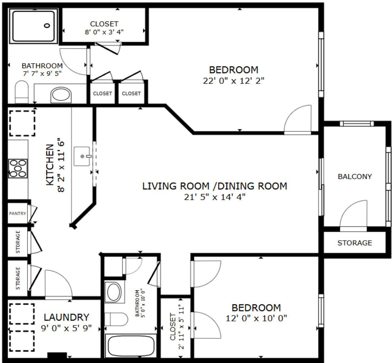
FLOOR PLAN
